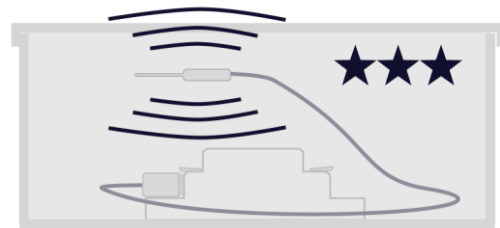
Figure 10: Freely place the antenna in a plastic junction box / housing (not against plastic)
