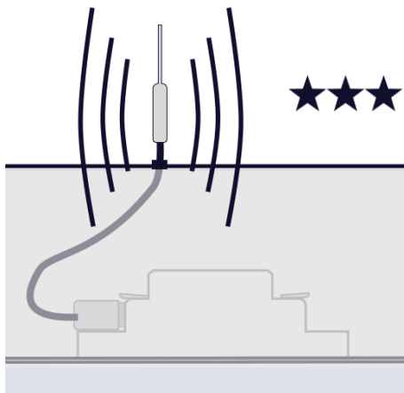
Figure 2: Route the thickened part of the antenna completely through the metal housing / cabinet plus 1.5cm of the antenna cable.
